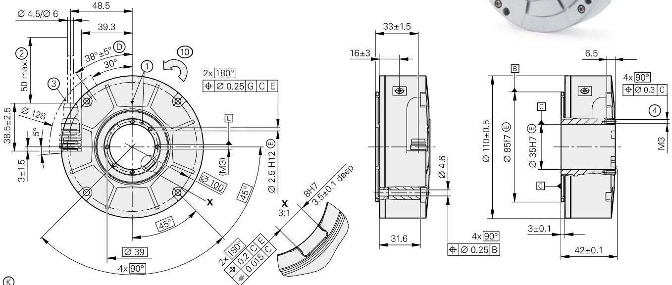
Shaft coupling with ring nut and catch With mechanical fault exclusion (for further dimensions, see "Without mechanical fault exclusion")
